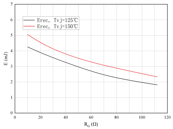
图 8. 开关损耗 二极管 Figure 8. Switching losses of Diode IF=60A, VCE=600V
